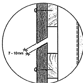
DETAIL 12.
