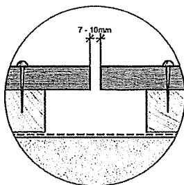
DETAIL 9.
