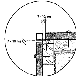
DETAIL 6.
