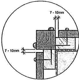
DETAIL 4.
