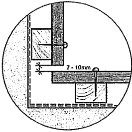
DETAIL 7.
