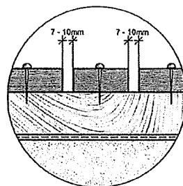
DETAIL 10.
